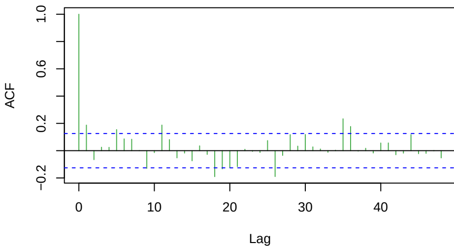
ACF – First Differenced
