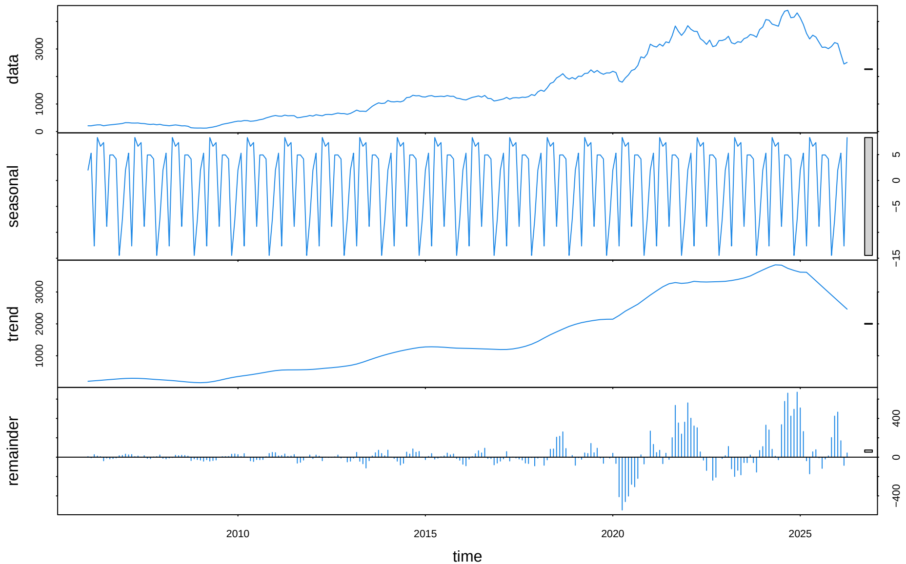
TCS Stock – STL Decomposition
