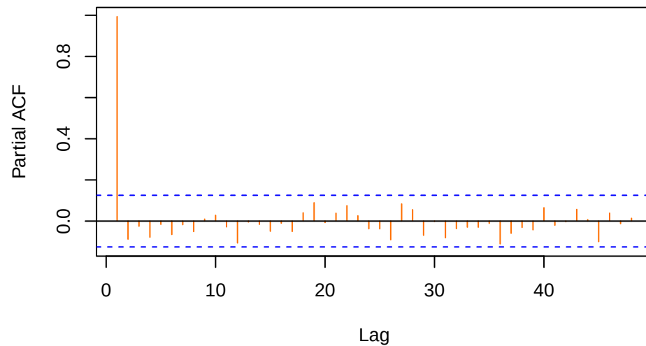
PACF – First Differenced
