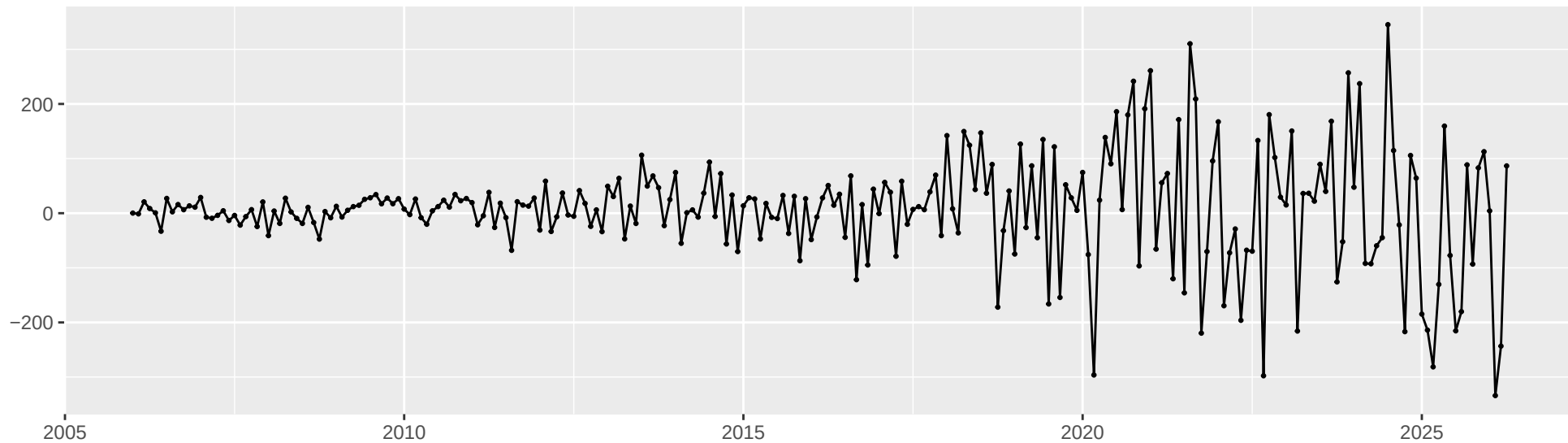
Residuals from ARIMA(1,1,1)(1,0,1)[12]
