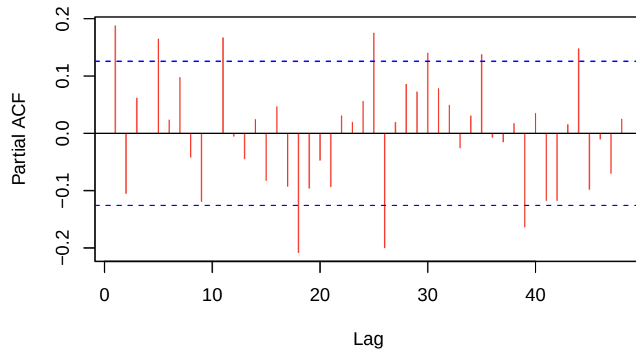
PACF – First Differenced
